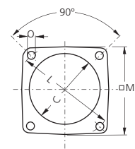
Connection M42 x 2 for ventilating filter
